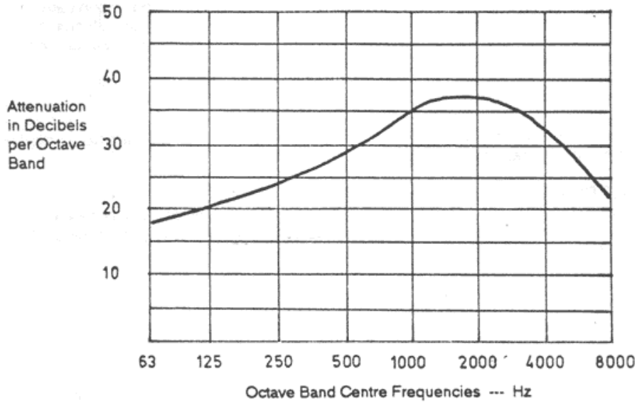
Typical Noise Attenuation Graph
